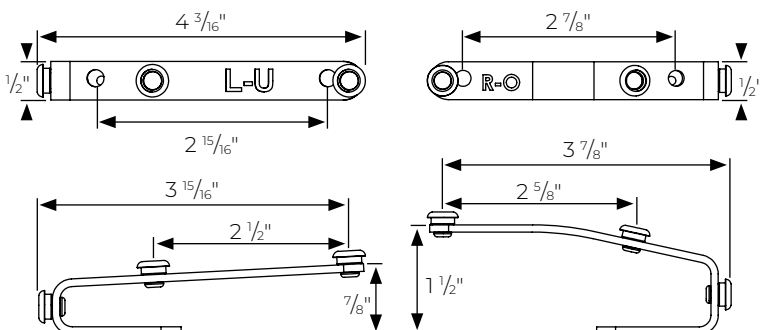
1 3/8" R-TEC Motorized Metal Traverse ONLY Pinch Pleat / Ripplefold Master Carrier Arms, Center Draw RTPTH138CD
