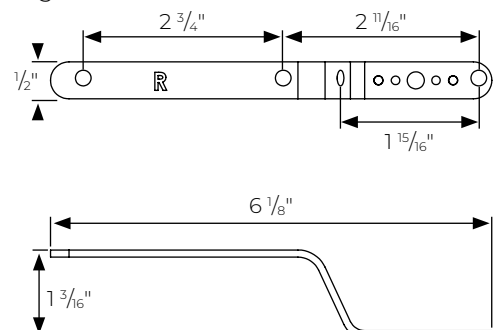
1 3/8" R-TEC Motorized Metal Traverse ONLY Pinch Pleat Master Carrier Arm, One-Way Draw Right - RTPTH138PPOR or Left - RTPTH138PPOL
