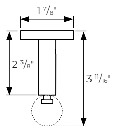
Ceiling Mount Single PTHMT138403
