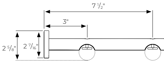
Wall Mount Double PTHMT138402
