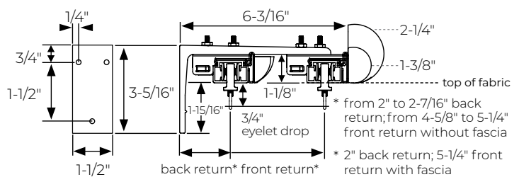
R-TEC Single or Double Motorized Bracket TB060-R
