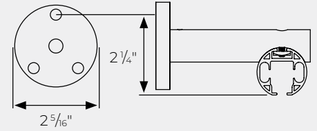
Wall Mount Bracket Mounting Plate
