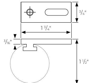
Low-Profile Single Ceiling PTHMT138406
