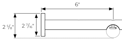
Wall Mount 6" return PTHMT138401
