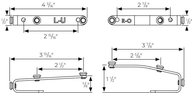
R-TEC Motorized Heavy Duty Traverse ONLY Universal Tandem Master Carrier Arms, Center Draw RTMDTCDTAN (see page 52 for details)
