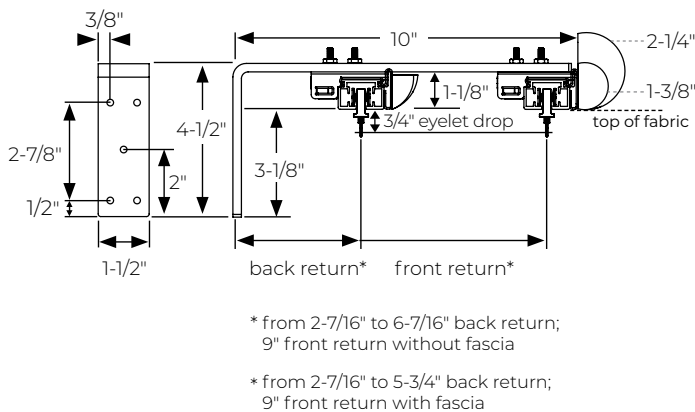
R-TEC Single, Double or Triple Motorized Bracket TB100-R
