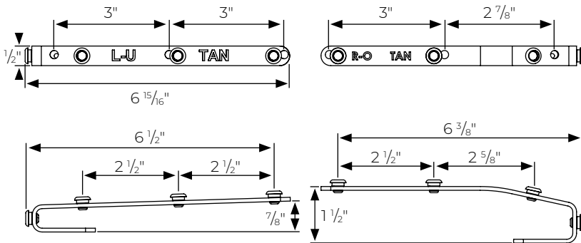
R-TEC Motorized Heavy Duty Traverse ONLY Universal Tandem Master Carrier Arms, Center Draw RTMDTCDTAN (see page 52 for details)
