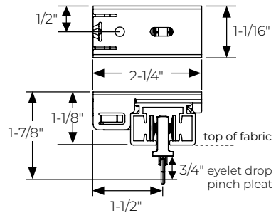
R-TEC Ceiling Mount Bracket RTMDTBCM
