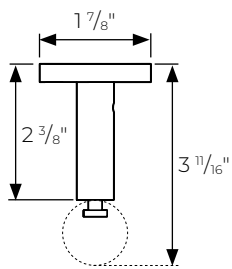
Ceiling Mount Single PTHMT138403
