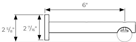
Hinged Elbow PTHMT138409
