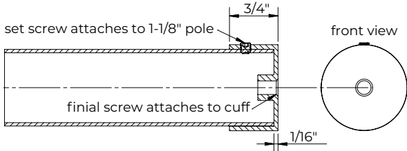
Transitional and Deco Cuffs / Finial Adapters
