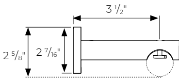
Wall Mount 3 1/2" return PTHMT138400
