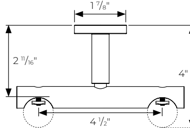
Ceiling Mount Double PTHMT138404
