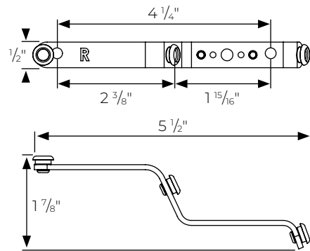
R-TEC Motorized Heavy Duty Traverse ONLY Ripplefold Butt Master Carrier Arm, One-Way Draw, Right or Left - RTMDTOB
