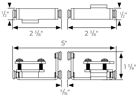
1 3/8" R-TEC Motorized Metal Traverse ONLY Pinch Pleat / Ripplefold Master Carrier Arms, Center Draw RTPTH138CD
