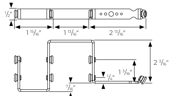
1 3/8" R-TEC Motorized Metal Traverse ONLY Pinch Pleat Master Carrier Arm, One-Way Draw Right - RTPTH138PPOR or Left - RTPTH138PPOL
