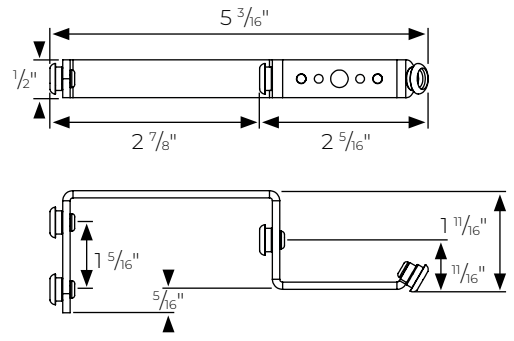
R-TEC Motorized Heavy Duty Traverse ONLY Ripplefold Butt Master Carrier Arm, One-Way Draw, Right or Left - RTMDTOB
