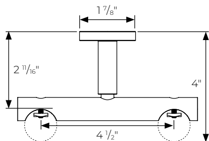
Ceiling Mount Double PTHMT138404
